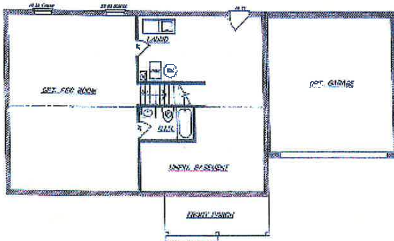
BASEMENT PLAN
